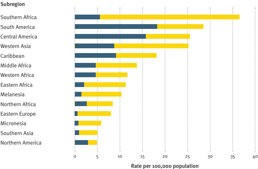
Figure 10 Average rates of violent death by firearm and other means, selected subregions, 2011–16
